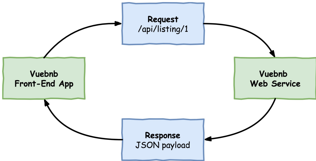
Figure 4.1. Vuebnb web service Web services are a speciality of Laravel, so it won't be hard to create one for Vuebnb. We'll use routes for our API endpoints and represent the listings with Eloquent models that Laravel will seamlessly synchronize with the database:
