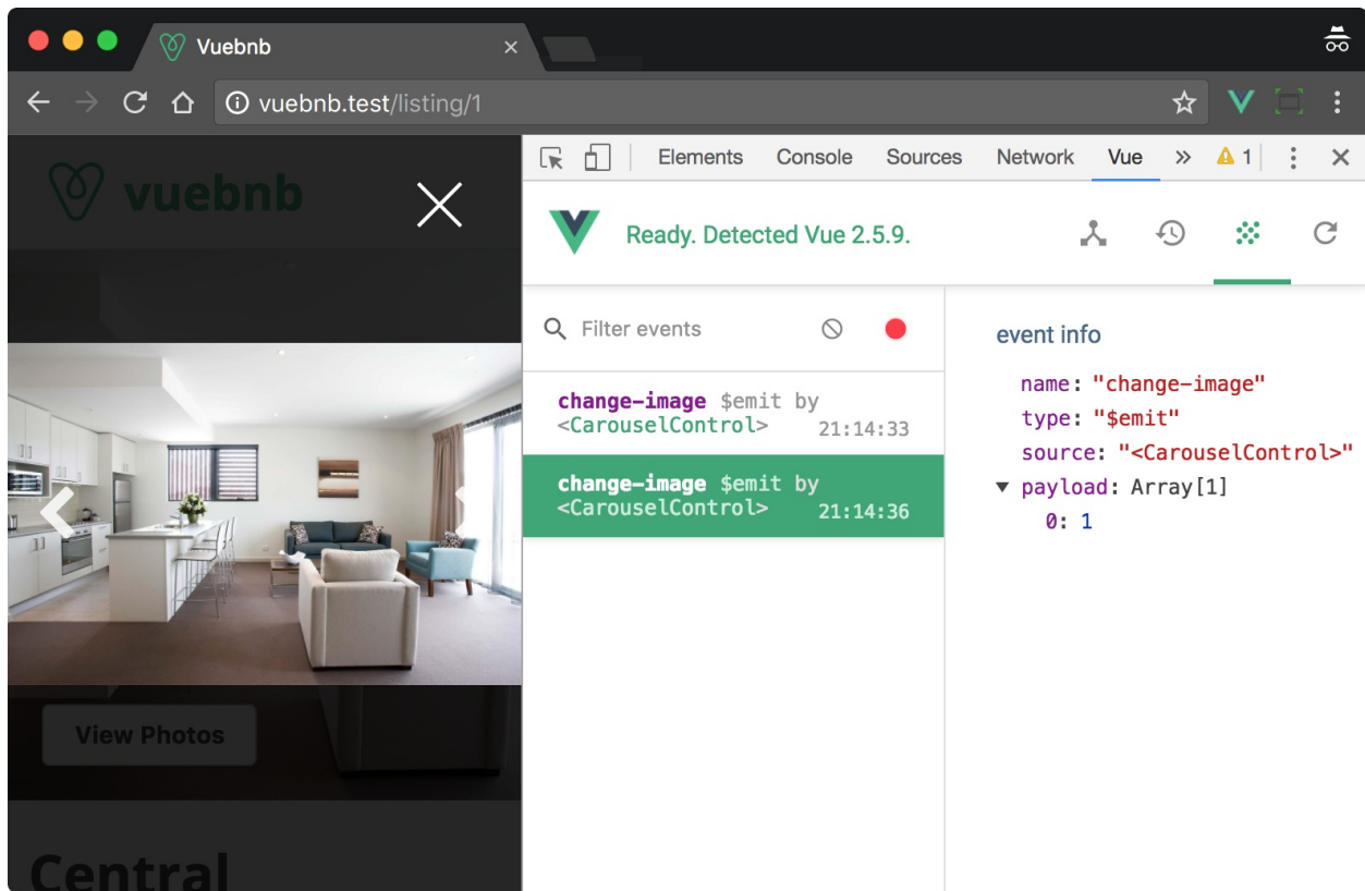
Figure 6.7. Screenshot showing a custom event and its payload ImageCarousel will now need to listen for the change-image event via the v-on directive. The event will be handled by a method changeImage which will have a single parameter, val , reflecting the payload being sent in the event. The method will then use val to step the value of index , ensuring it loops to the start or end if it exceeds the bounds of the array it indexes.
