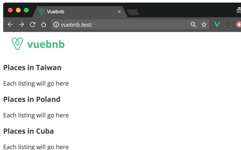
Figure 7.9. Iterating the listing summary groups in the HomePage component Since each listing summary will be of some complexity, we'll create a separate component, ListingSummary , for displaying them: $ touch resources/assets/components/ListingSummary.vue
