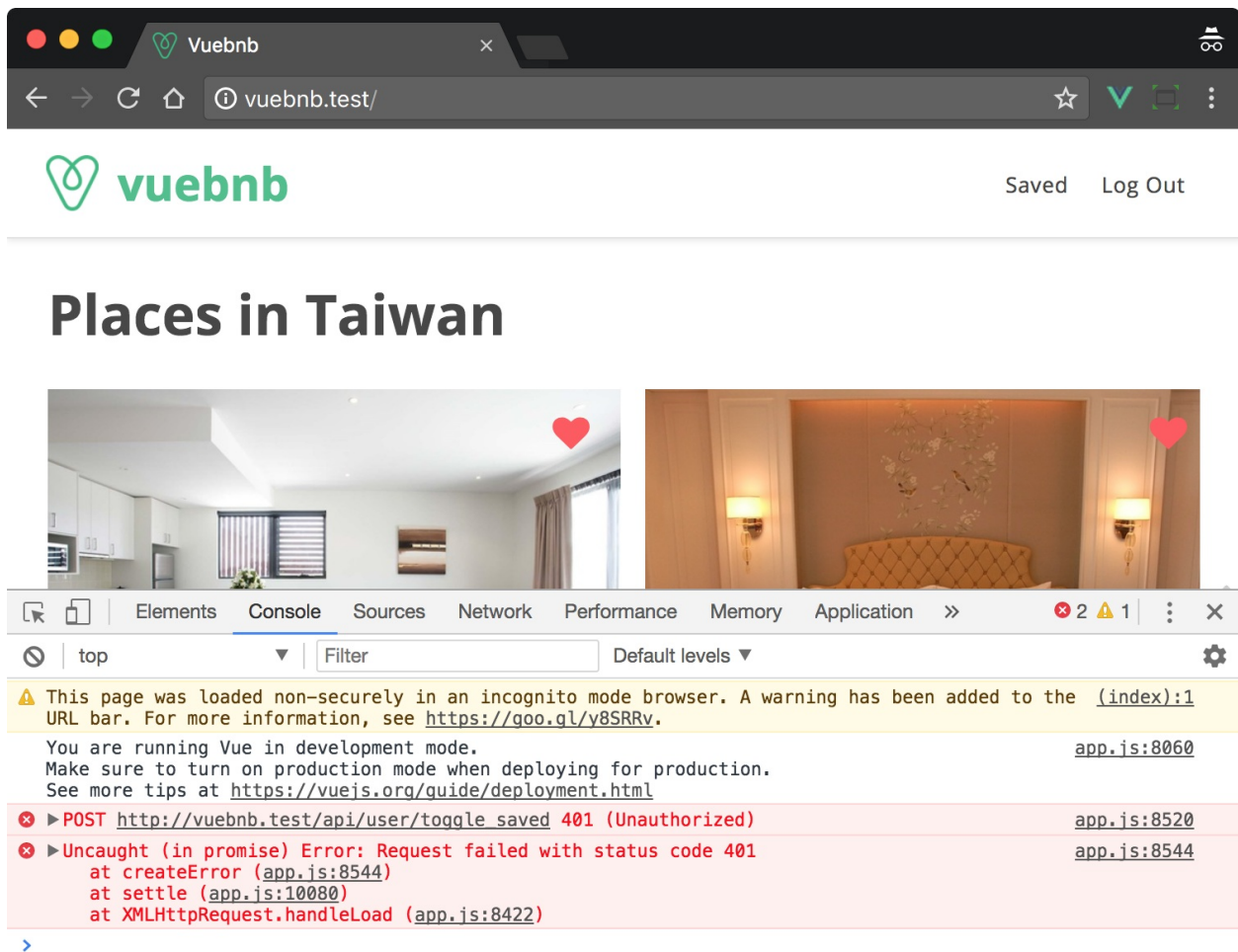
Figure 9.10. AJAX call results in a 401 Unauthenticated error
