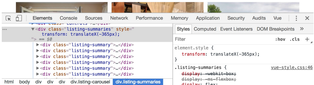
Figure 7.22. Listing group shifted to the left by using translate By binding inline style to the element with the listing-summary class, we can control the translate from JavaScript. Let's do this via a computed property so we can calculate the translate amount dynamically.
