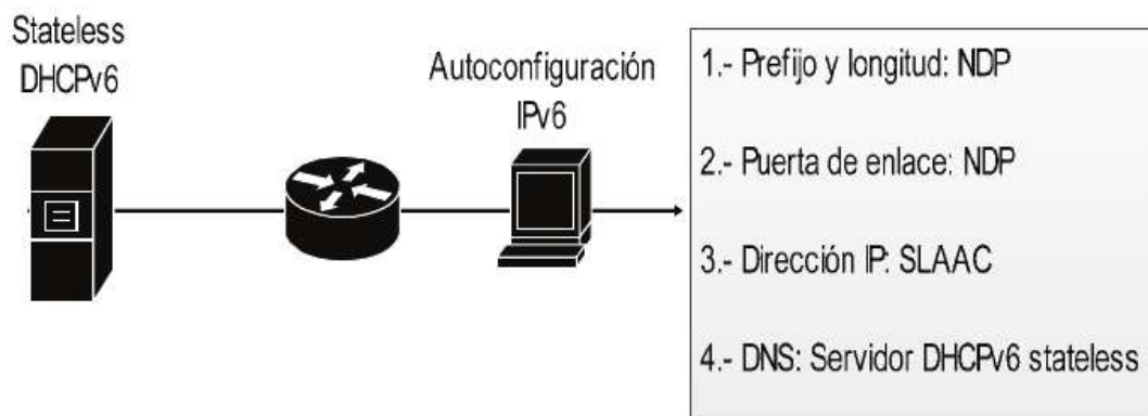
Fig. 11-12 Stateless DHCPv6.
