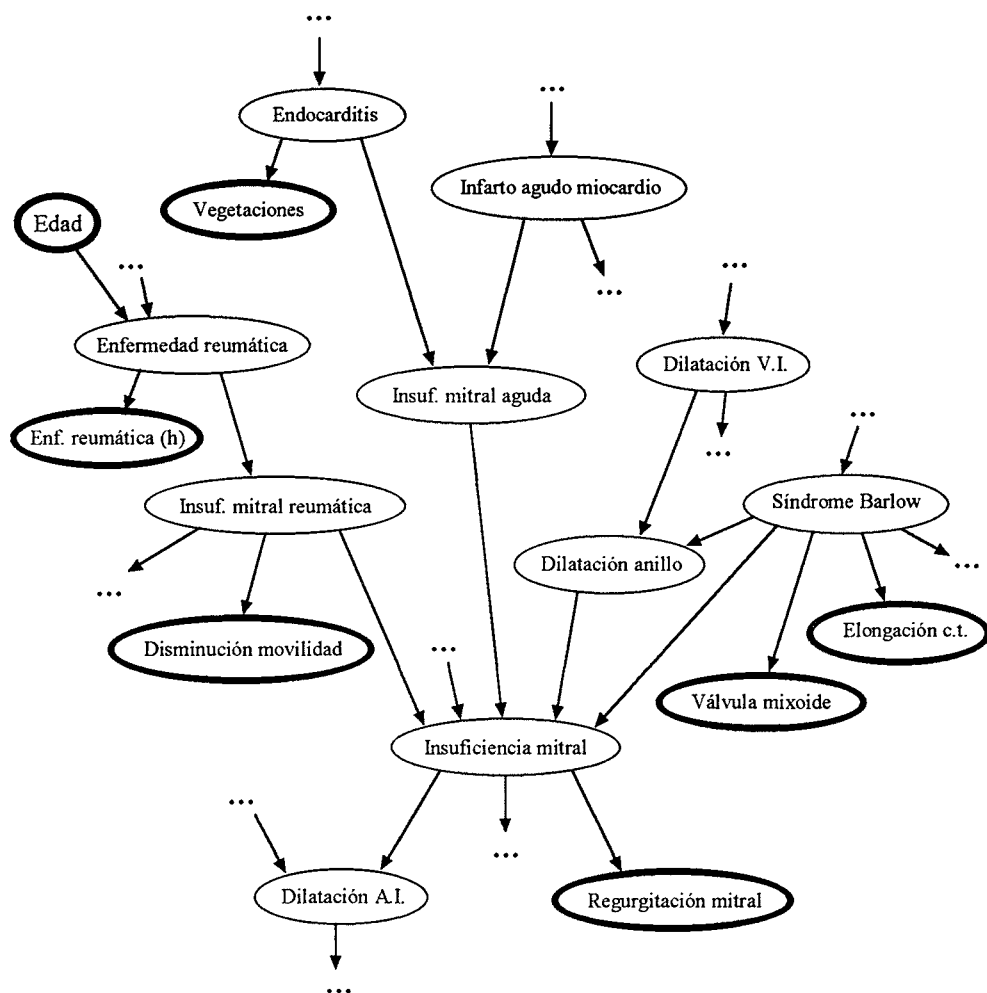
Figura 6-3 Red bayesiana de DIAVAL.
