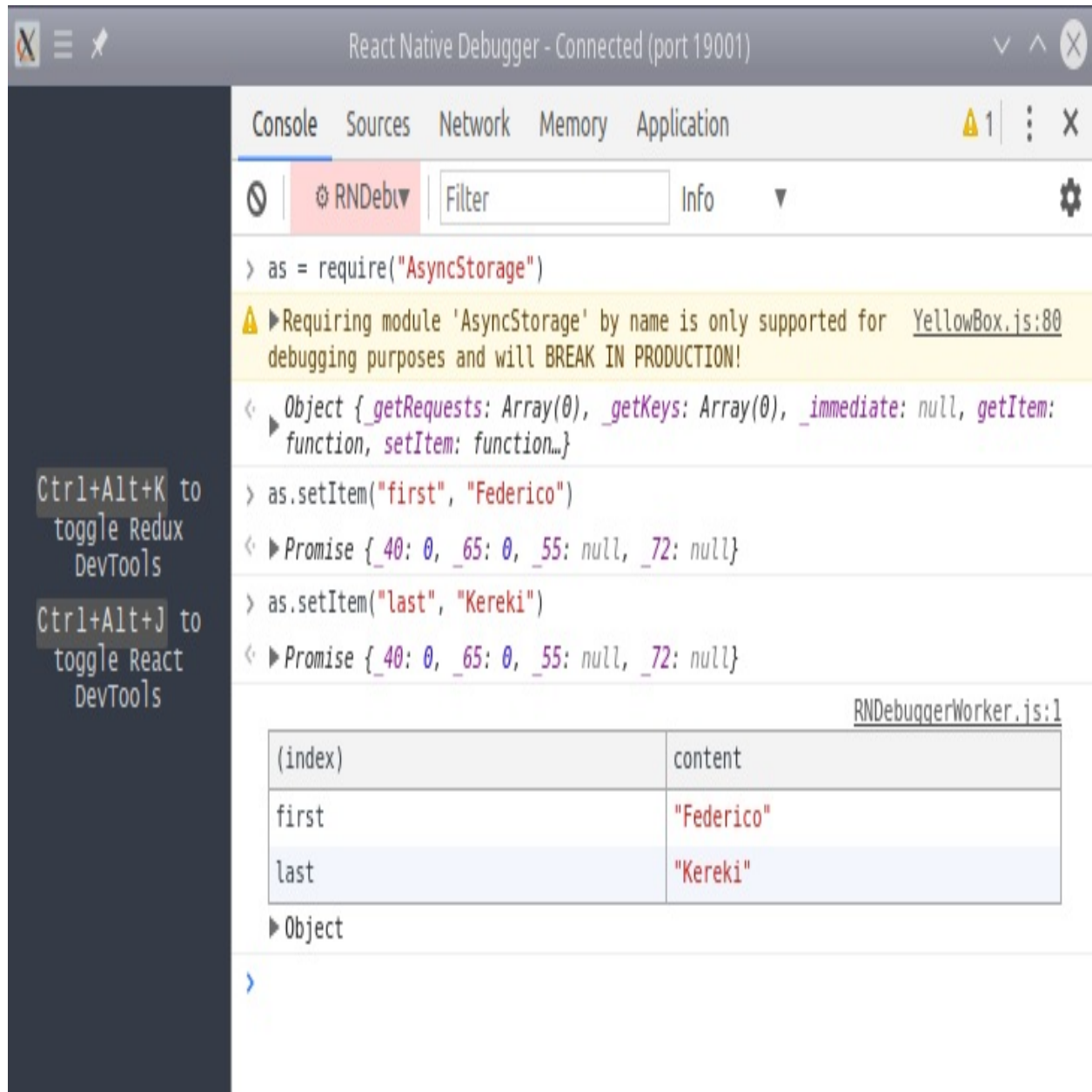
Examining AsyncStorage with the RN debugger
