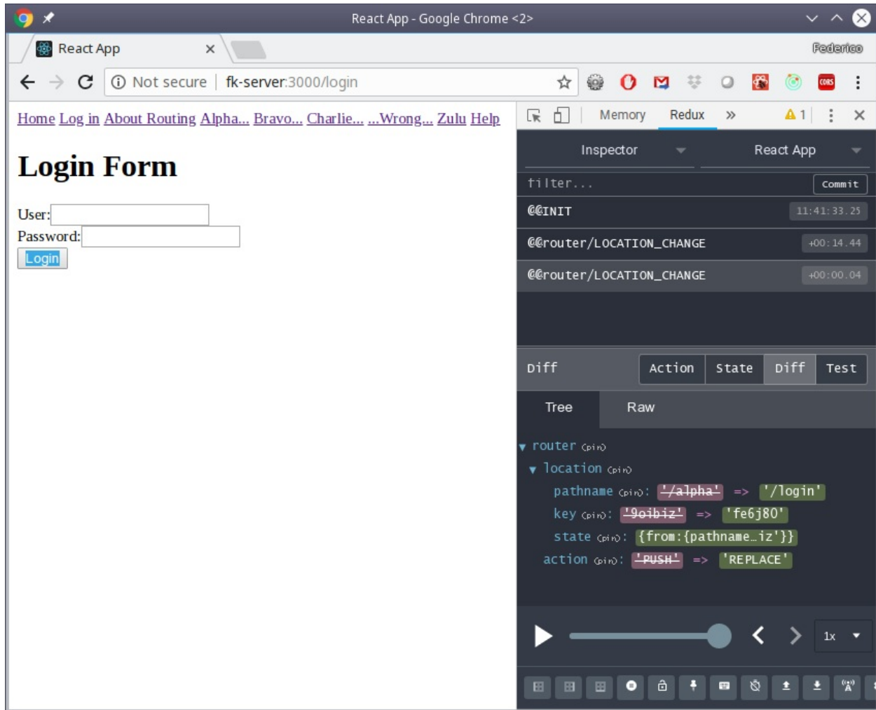
Attempting to access a protected route redirects us to the login page
