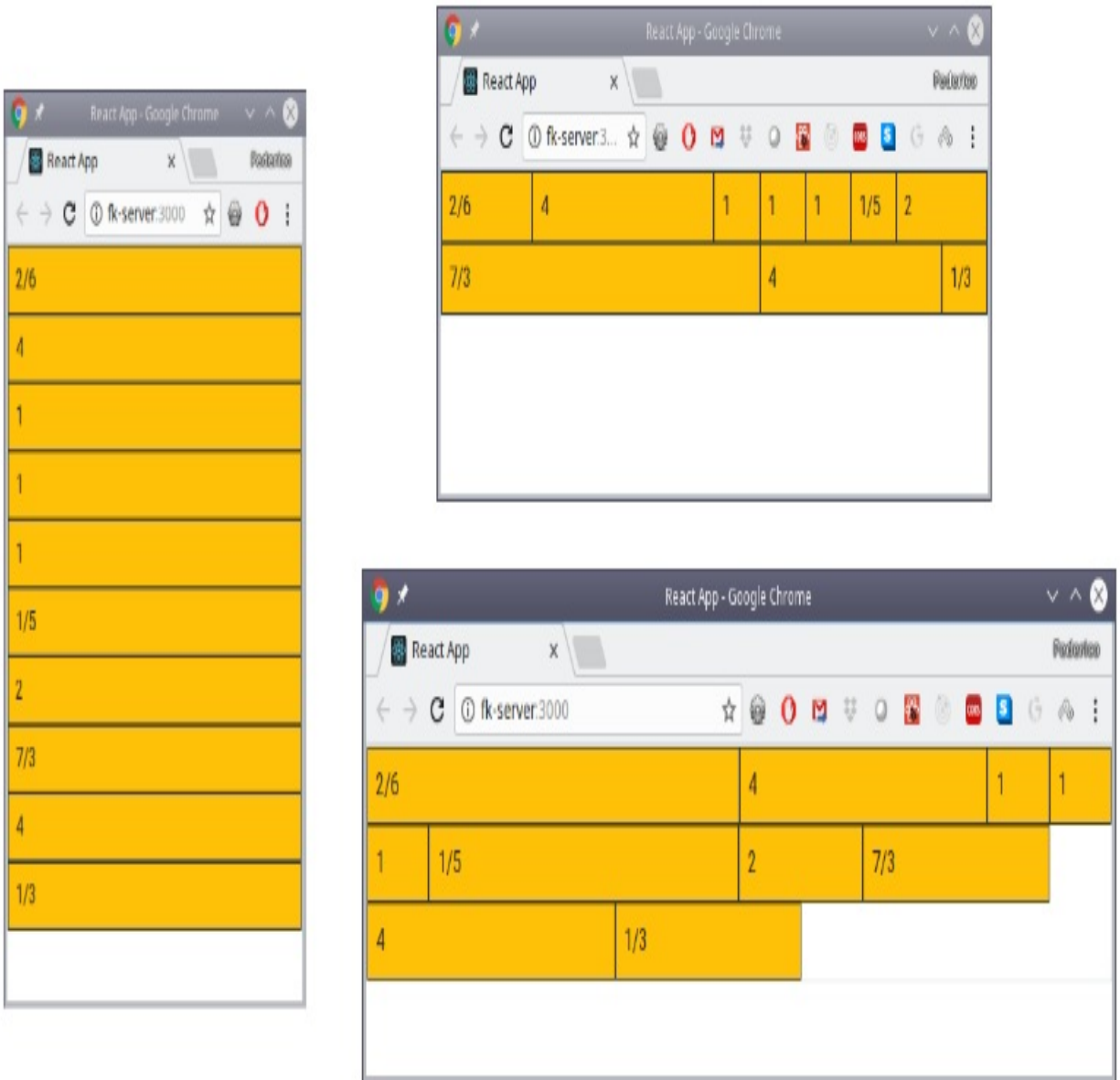
The same elements, rendered at different screen widths
