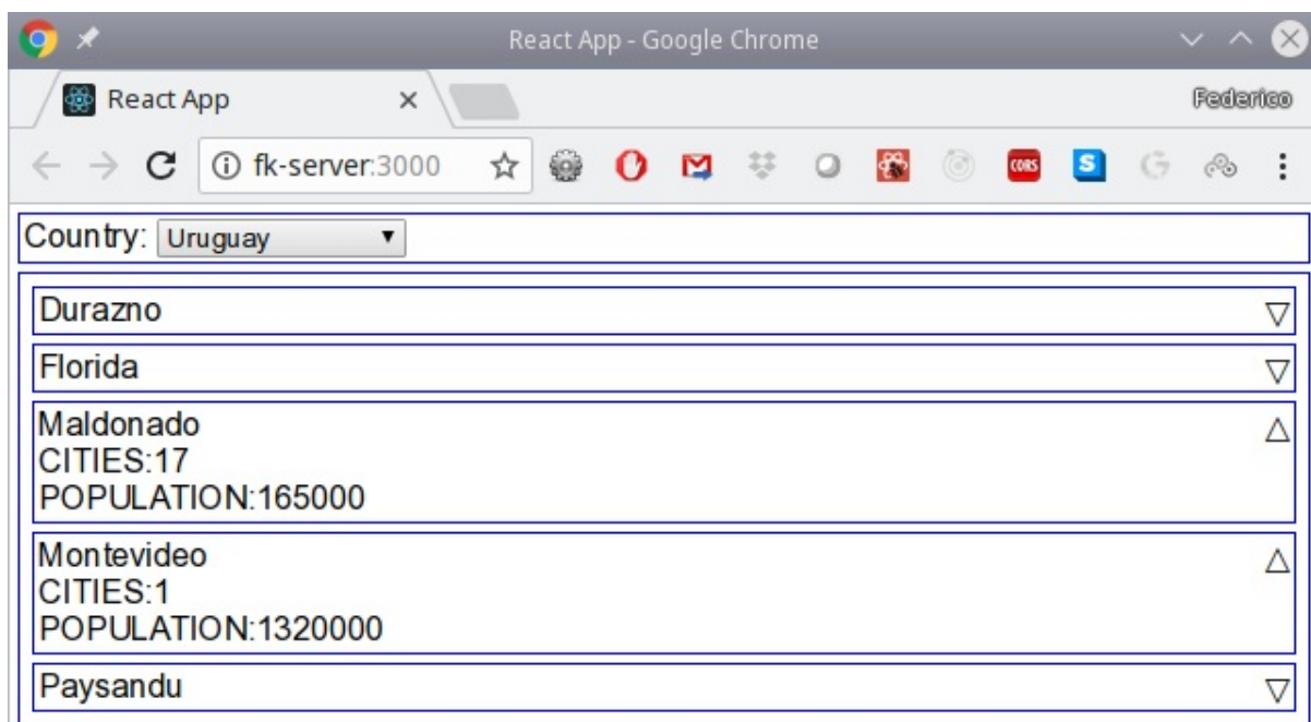
A run of our application; some cards are expanded and show their children
