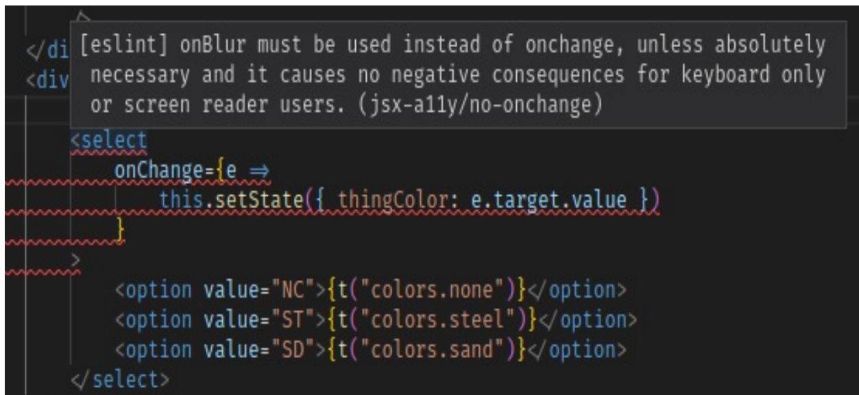
Our things ordering form only has a small a11y problem
