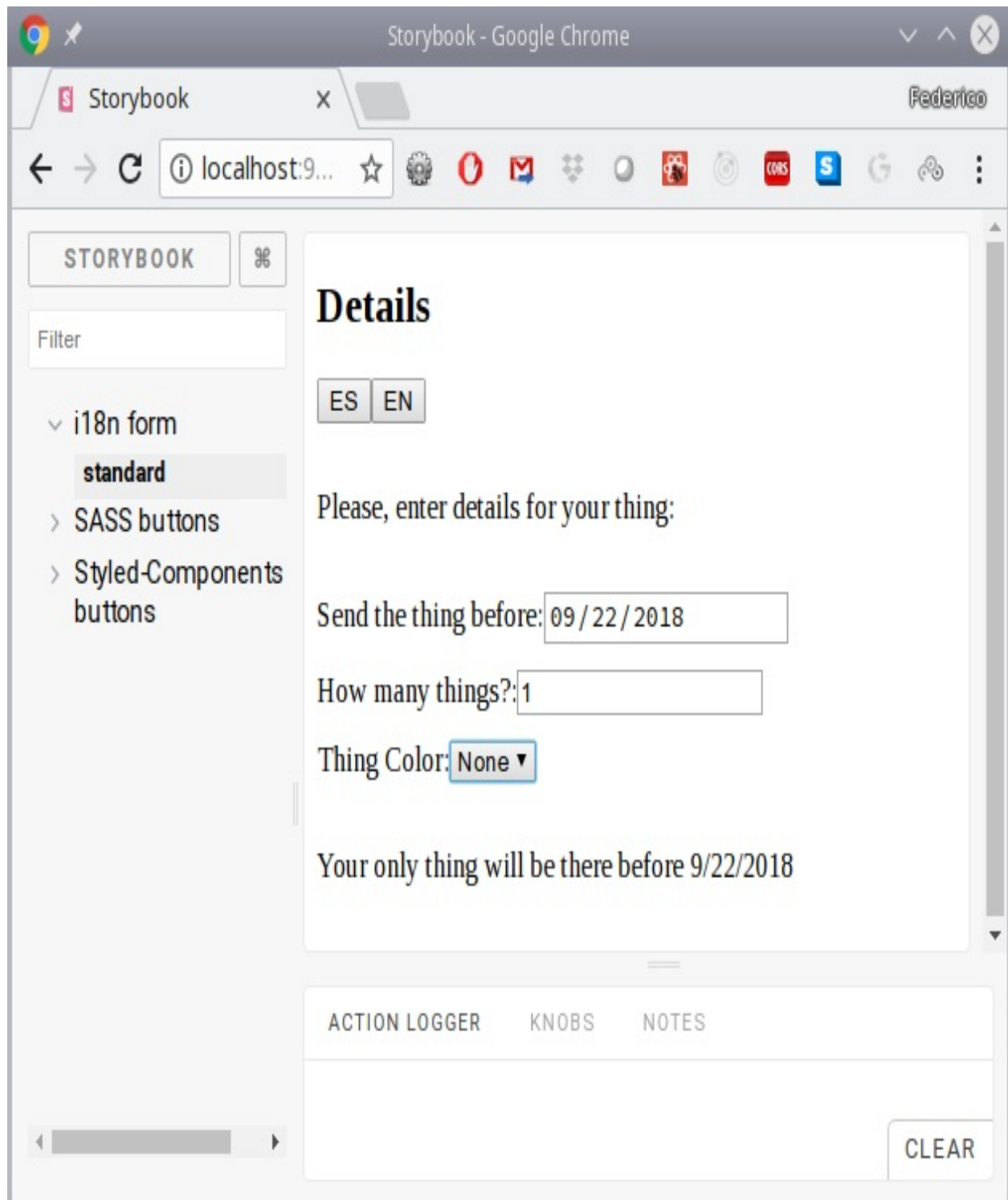
Our input form, with initial values, displayed in English
