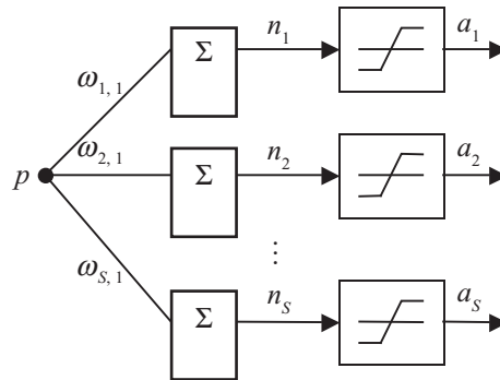
Fig. 3.46 Red Outstar.
