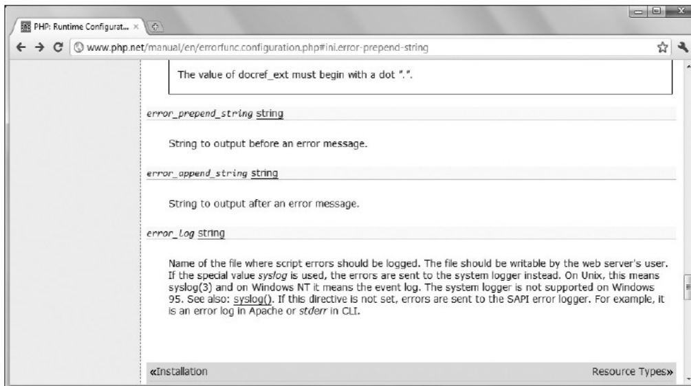
Figura 10. Directiva error_prepend_string .
