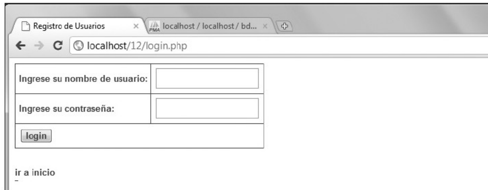
Figura 4. login.php.
